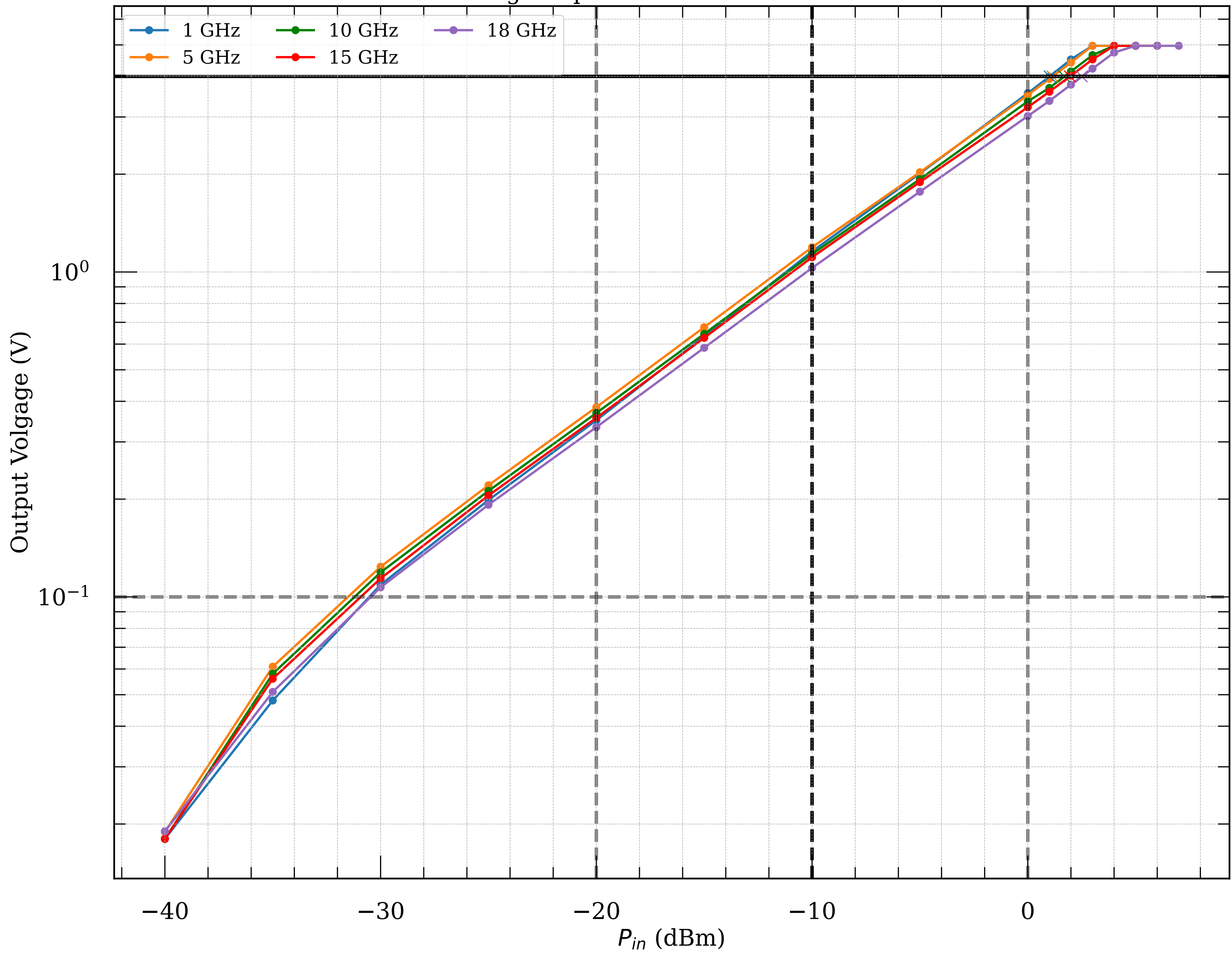
Measured voltage-to-power curve of detector module022v2
